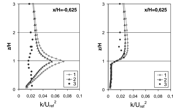
Figure 3. Comparison of the profile of the turbulent kinetic energy observed in the wind tunnel with predictions at x/H = -0.625 and x/H = 0.625 at y/H = 0 (- denotes upstream the cube centre). Numbers correspond to: 1 - standard k-\varepsilon model; 2 - Chen&Kim model; 3 - experimental data
