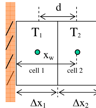
Figure 7. Scheme of grid cells attached to a vertical wall as treated in CHENSI
