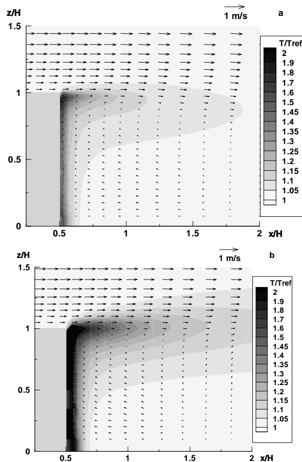
Figure 13. Velocity vectors and contours for temperature difference between wall and ambient air different "heated cube" cases with values Gr/Re^2 \approx 0.9 (a) and Gr/Re^2 \approx 1.6 at central cube plane y/H=0 .
