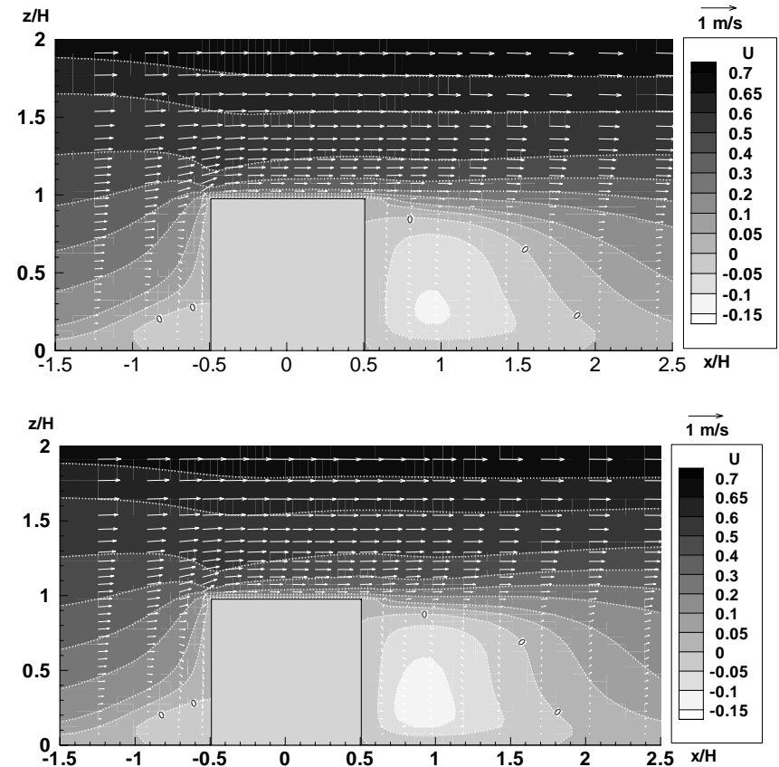
Figure 9. Vectors and contours for u velocity component for "heated cube" with values Gr/Re^2 \approx 1 (a) and Gr/Re^2 \approx 1.5 (b).
