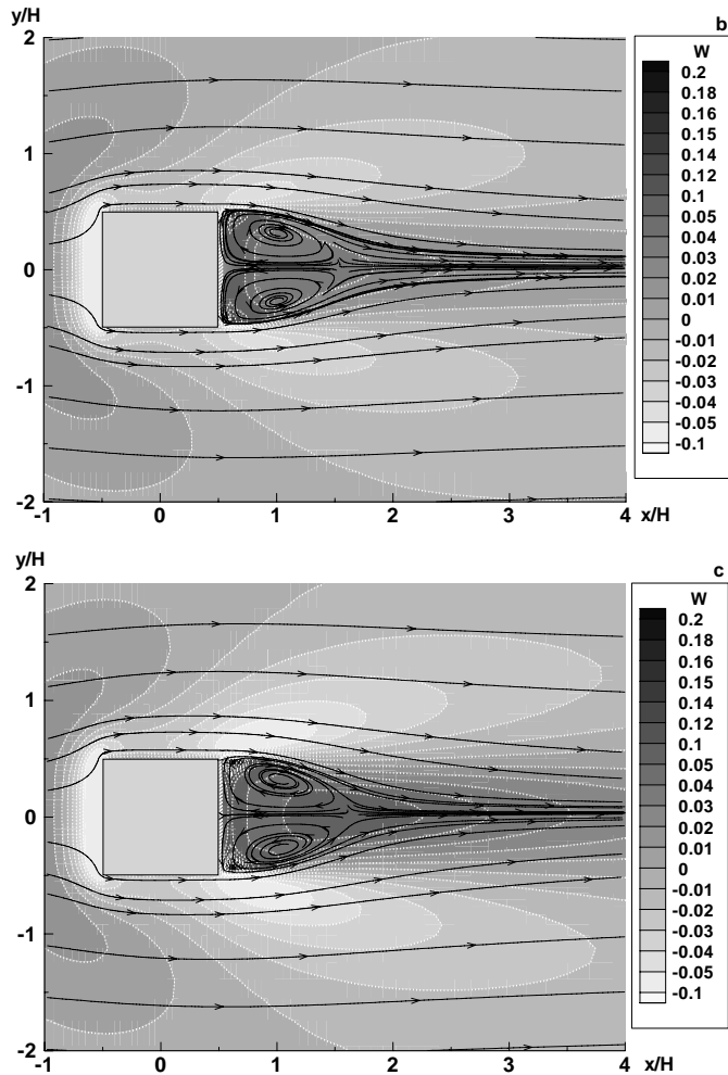
Figure 12. Horizontal plots of vertical velocity field for "cold cube" (a) and "heated cube" with values Gr/Re^2 \approx 0.9 (b) and Gr/Re^2 \approx 1.6 (c) at level z/H=0.75
