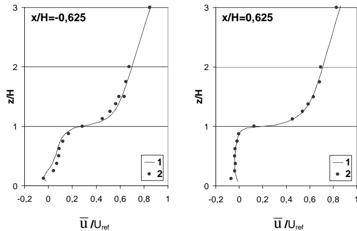
Figure 6. Comparison of the profile of the u velocity component observed in the wind tunnel with predictions at x/H=-0.625 and x/H=0.625 at y/H=0 (- denotes upstream the cube centre). Numbers correspond to: 1 - model data; 2 - experimental data.
