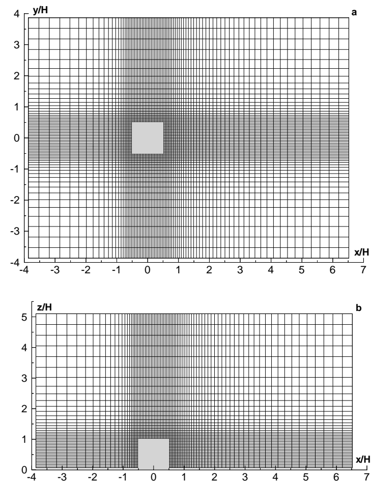
Figure 2. Computational mesh - horizontal (a) and vertical (b) cross section
