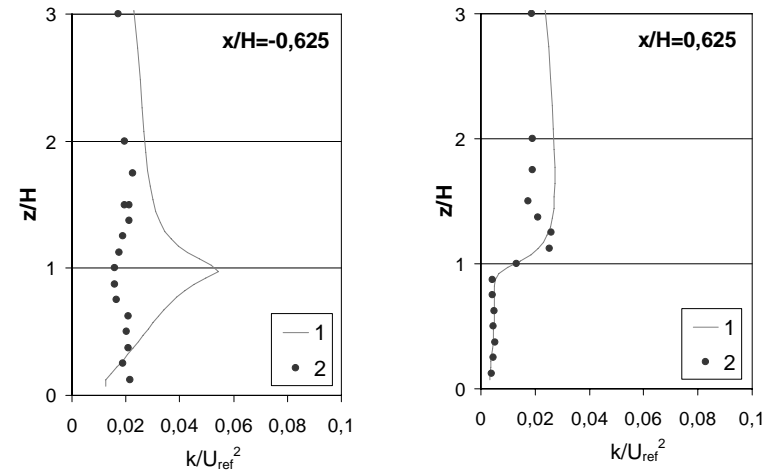
Figure 7. Comparison of the profile of the turbulent kinetic energy observed in the wind tunnel with predictions at x/H=-0.625 and x/H=0.625 at y/H=0 (- denotes upstream the cube centre). Numbers correspond to: 1 - model data; 2 - experimental data
