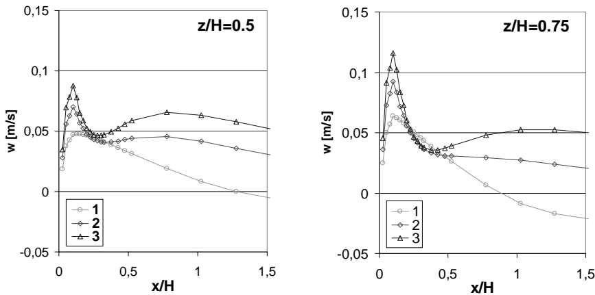
Figure 11. Vertical velocity plots at different levels at cube centre plane ( y/H=0 ). Numbers correspond to: "cold cube" (1), "heated cube" with value Gr/Re^2 \approx 0.9 (2) and Gr/Re^2 \approx 1.6 (3).
