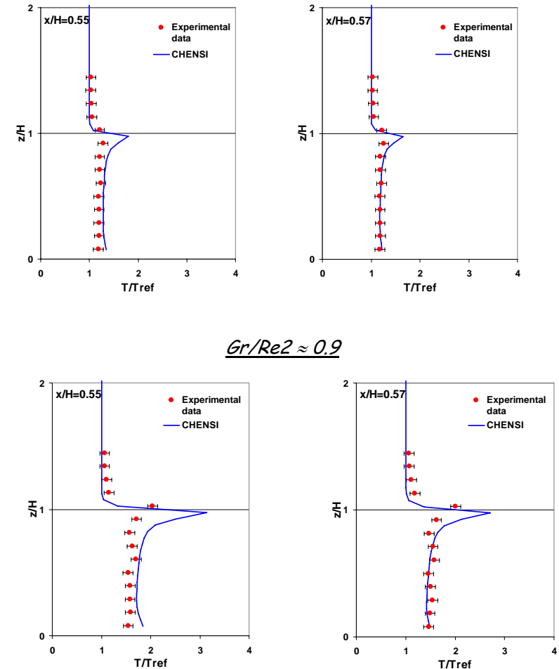
Figure 8. Vertical profiles of non-dimensioned temperature
