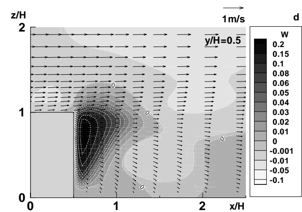
Figure 10. Contours for vertical velocity and velocity vectors for "cold cube" (a); "heated cube" with values Gr/Re^2 \approx 0.9 (b) and Gr/Re^2 \approx 1.6 (c) at cube centre plane y/H=0 ; "heated cube" with value Gr/Re^2 \approx 1.6 at y/H=0.5 (d).
