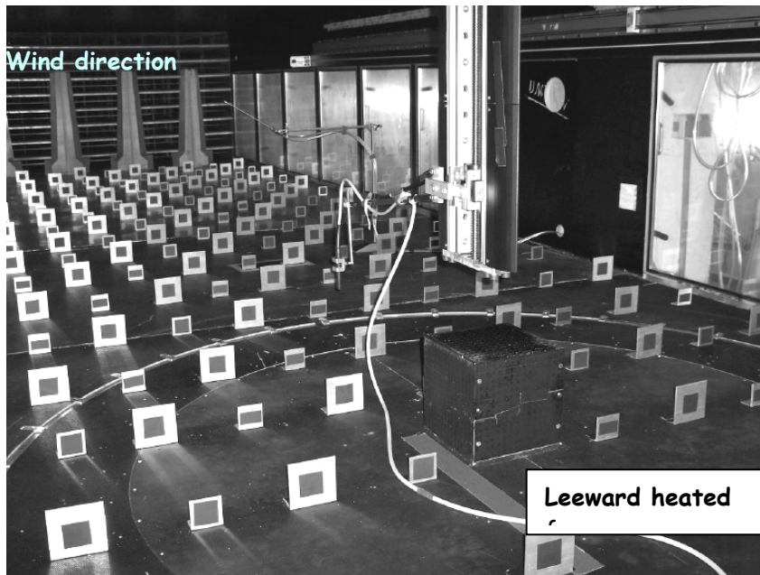
Figure 1. Physical model set-up
