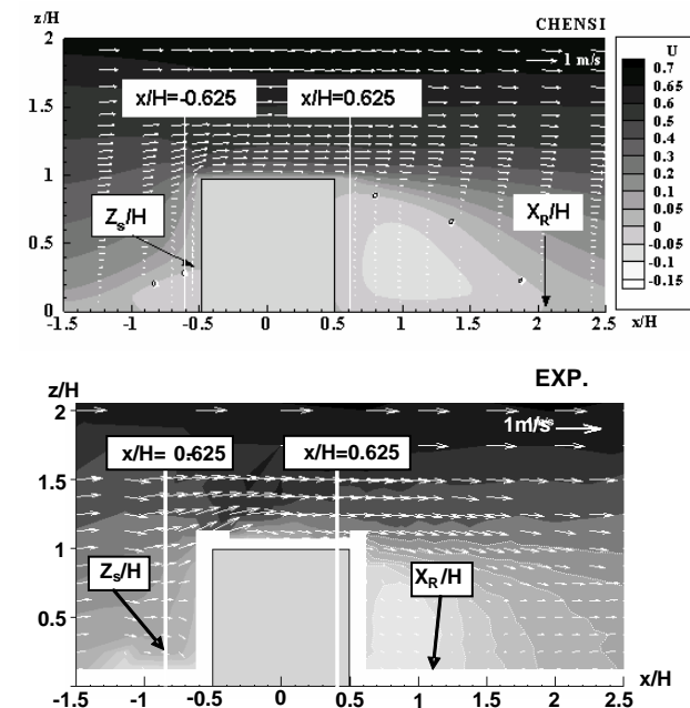
Figure 5. Vertical cross section of the dimensionless u component normalized with the free-stream velocity ( U_{ref}=1m/s )
